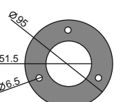
7051 95x51.5 □ 4
